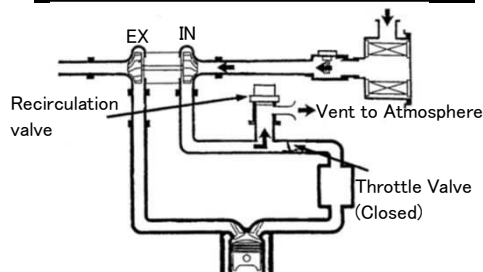
Re-Circulation Vent to Atmosphere Valve
