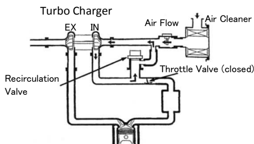
Standard Re-Circulation Valves
