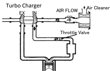
Standard Re-Circulation Valves
