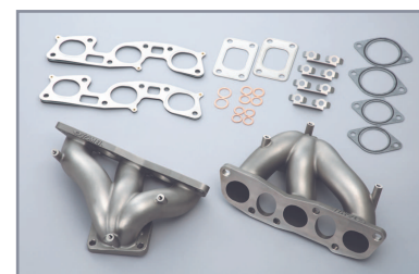
FULL CAST EXHAUST MANIFOLD P/N:415003
