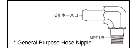
#8 Elbow 1/8NPT PART # : 185104
