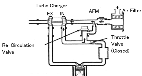
Standard Re-Circulation Valves
