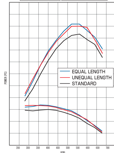
ENGINE DYNO RESULTS ENGINE TYPE EJ25 PURPOSE HEADER COMPARISON BOOST SETTING Gain 70 SPECS EJ25 STANDARD ENGINE
